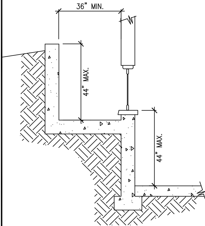
CROSS SECTION
