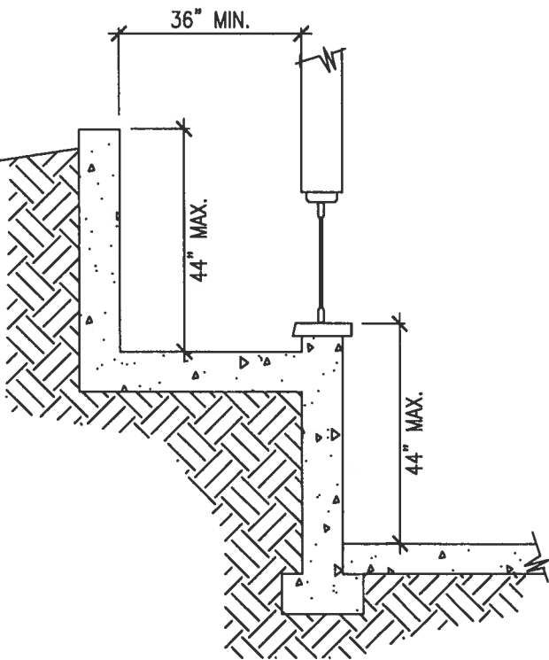
CROSS SECTION
